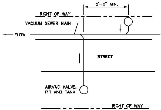
MINIMUM SPACING BETWEEN CONNECTIONS
