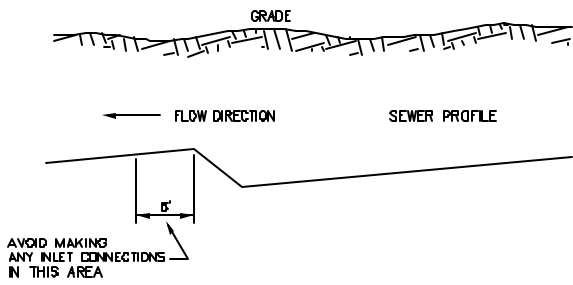
CONNECTION LOCATIONS TO AVOID
