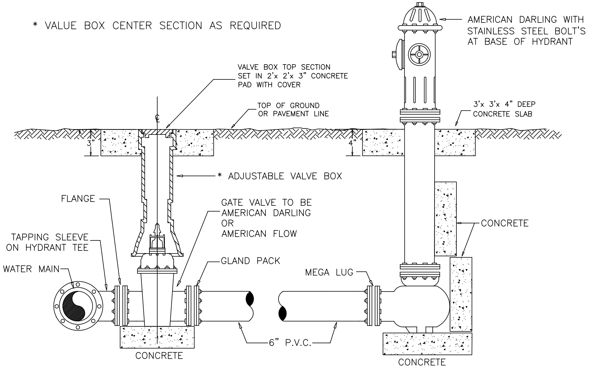
TYPICAL FIRE HYDRANT ASSEMBLY
