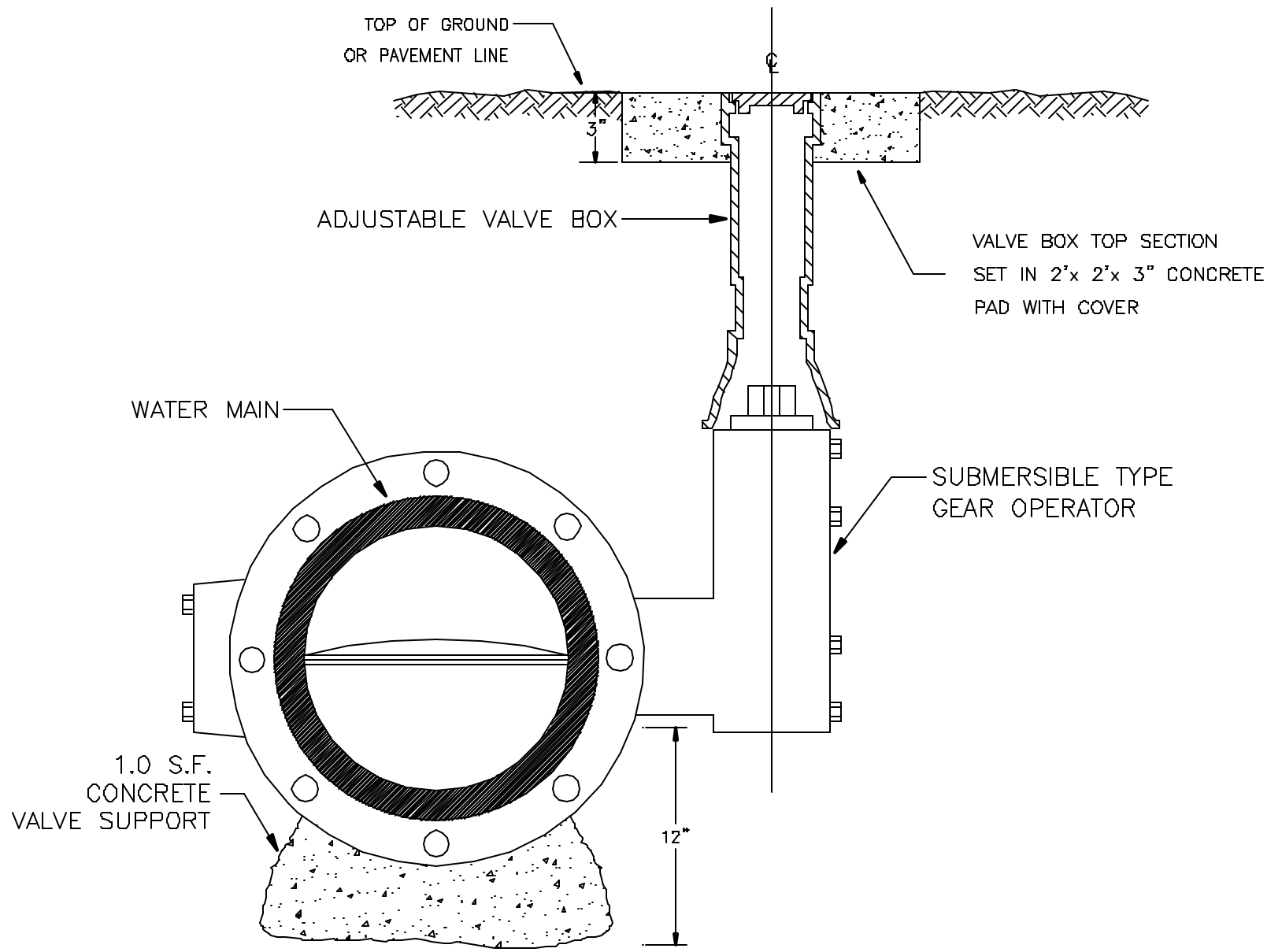
TYPICAL BUTTERFLY VALVE DETAIL
